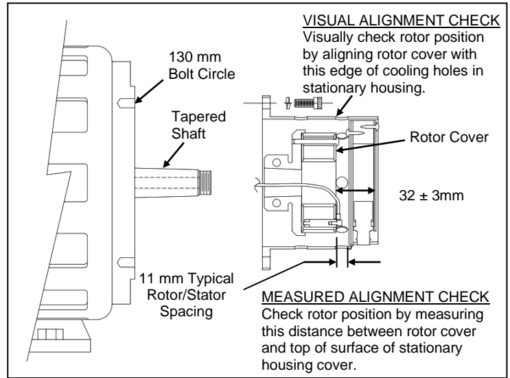
Installation Diagram
