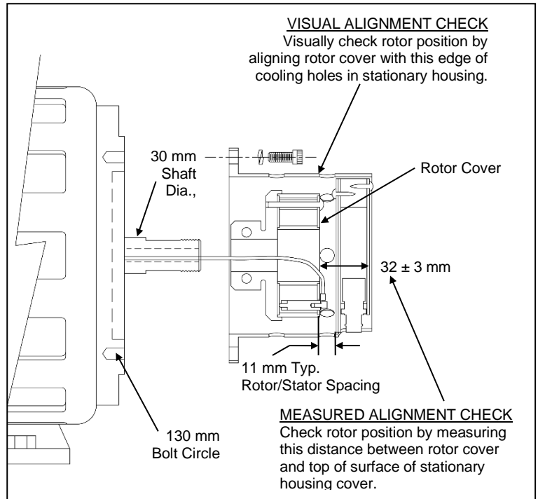
Installation Diagram
