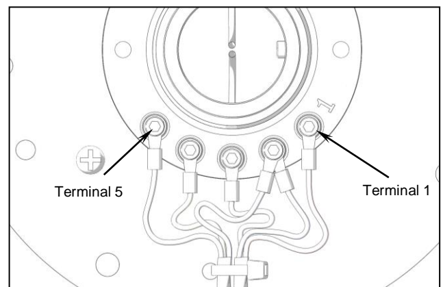
Stator Wiring Diagram
